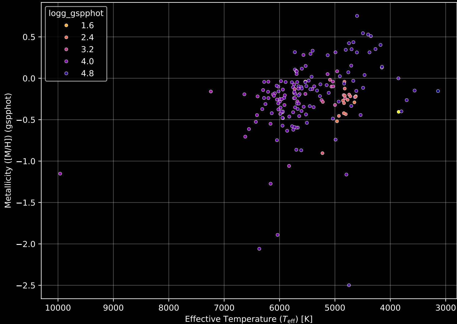
APOGEE DR17 Field: [136+71_MGA] Stellar Population Parameters (n= 177)
