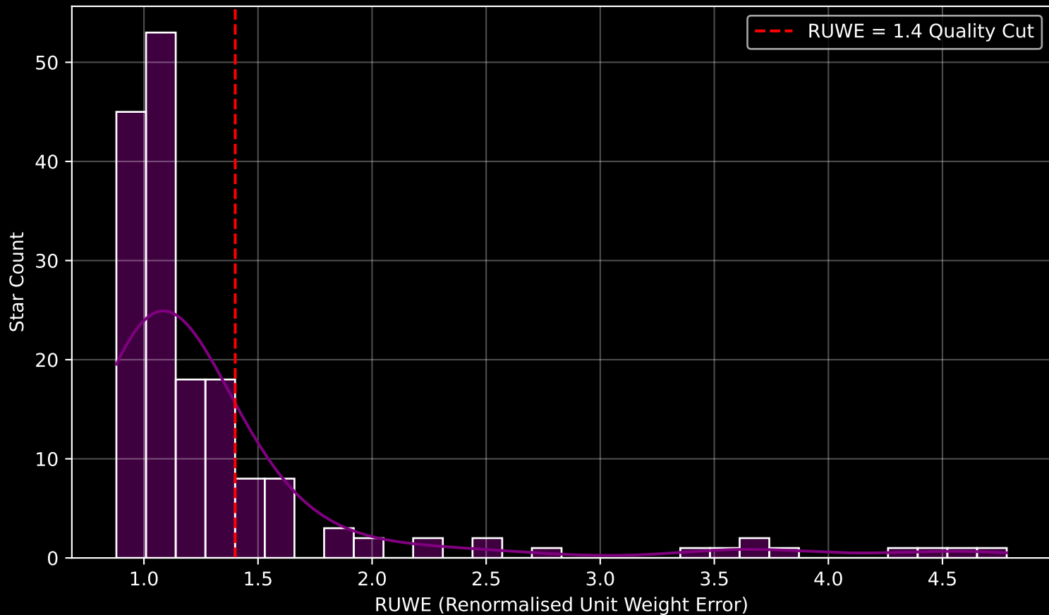
GAPOGEE DR17 Field [136+71_MGA] RUWE Distribution (n= 169)
