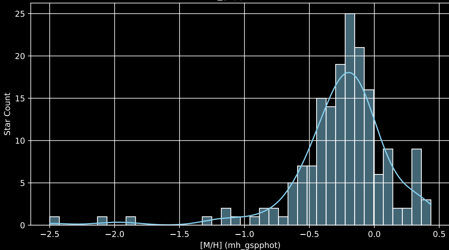
APOGEE DR17 Field: [136+71_MGA [M/H] (mh_gspphot) (n= 173)
