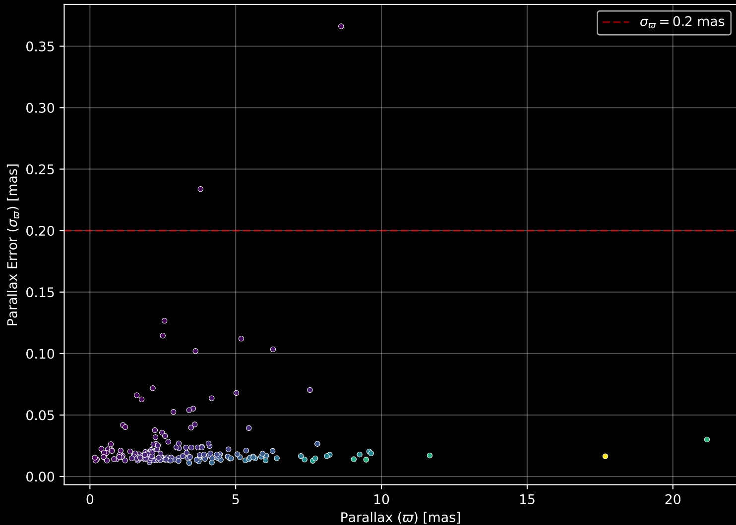
APOGEE DR17 Field: [136+71_MGA] Parallax Quality (n= 177)
