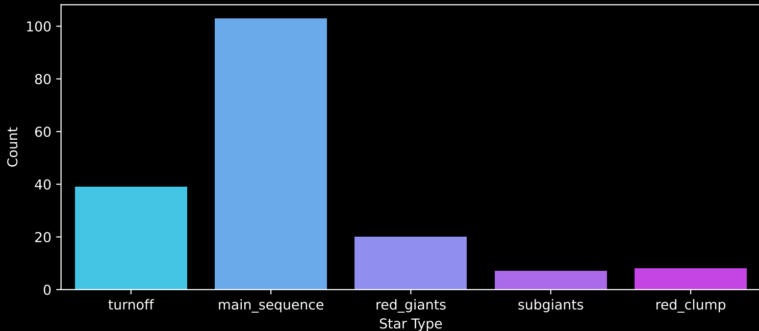
APOGEE DR17 Field: [136+71_MGA] Count plot of Star Type
