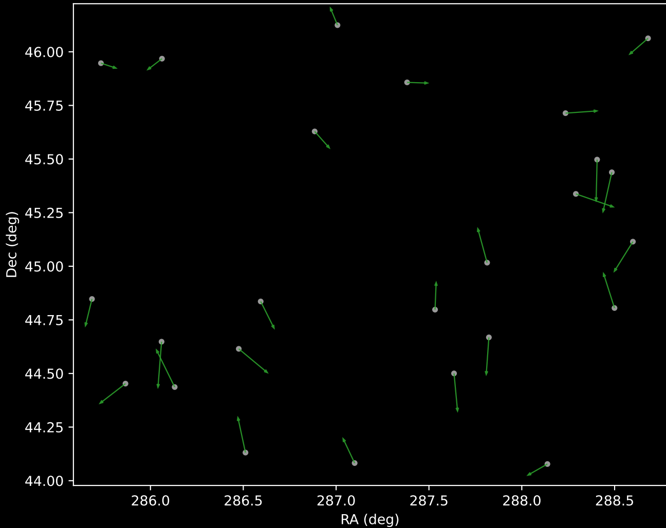
APOGEE DR17 Cluster 4 Proper Motion Vectors (n=25)
