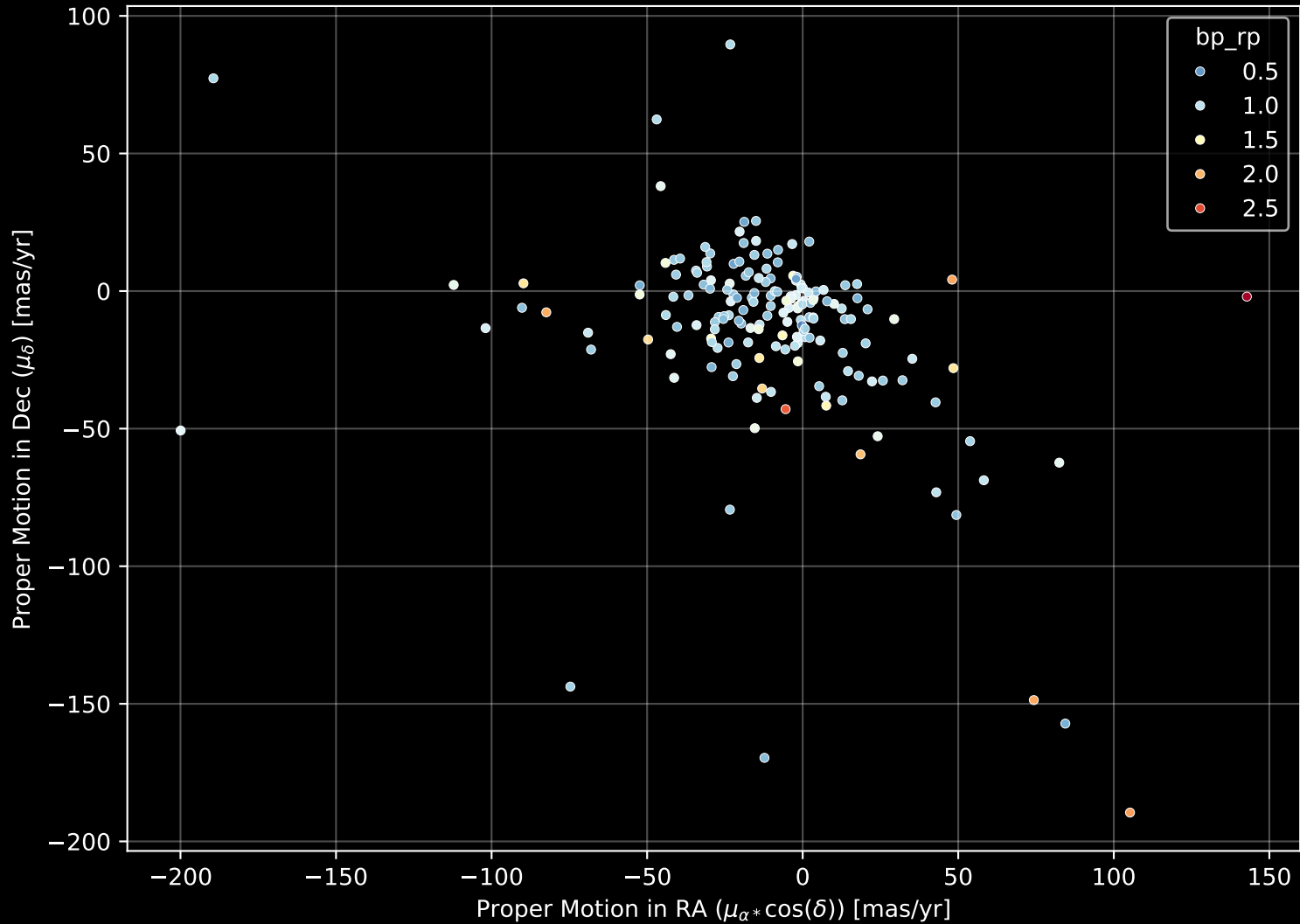
APOGEE DR17 Field: [136+71_MGA] Proper Motion Diagram (n= 177)
